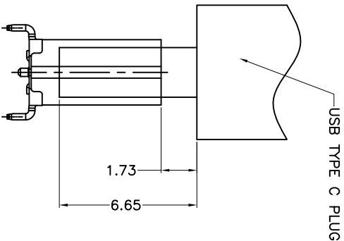
FEMALE AND MALE MATCHING DRAWING
